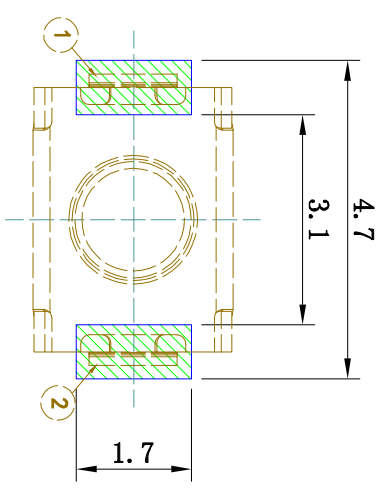
P.C.B MOUNTING PATTERN DIMENSION
